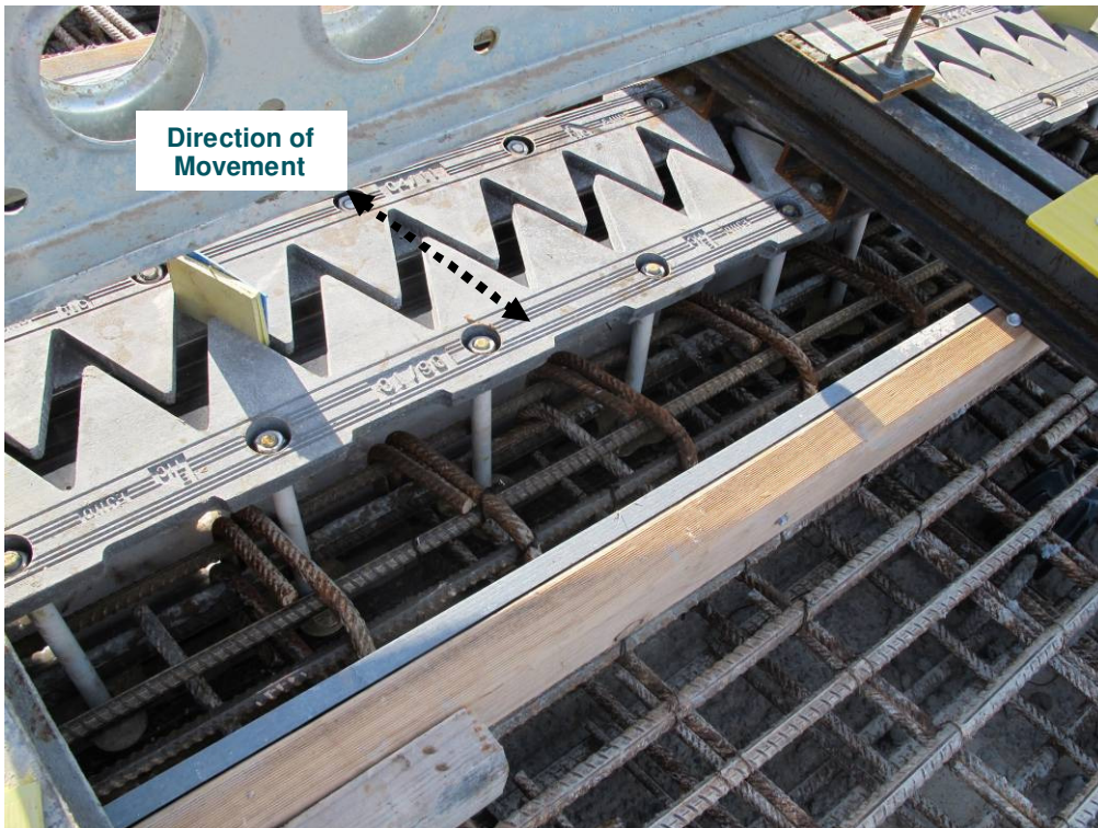
Granor Etic® EJ110 aluminium saw-tooth joint being installed into block-out. Teeth are offset slightly in transverse direction to allow for skewed line of movement.
